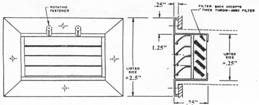
FILTER BACK
